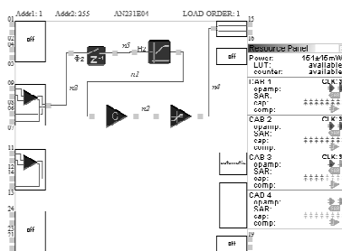
Fig. 6. A schematic of the infinite limiter
