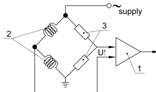
Fig. 4. Schematic diagram of the measurement bridge with an inductive sensor, 1 – ac current amplifier, 2 – coils, 3 – resistors, U – bridge output voltage.
