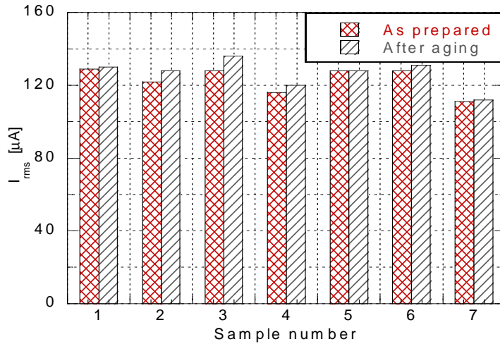
Fig. 6. Changes of the leakage current I_{rms} in an exemplary set of seven varistors at a polarizing voltage of 350 Vrms before and after aging by applying 1000 current pulses of amplitude 0,5 kA and duration 8/20 \mu\text{s} .
