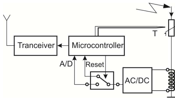
Fig. 9. Measurement system for varistor quality monitoring.
