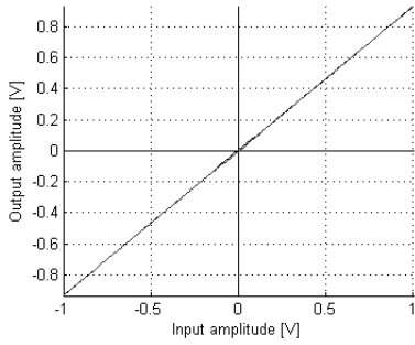
Fig. 6. Transfer function of amplifier I .
