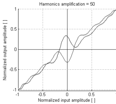
Fig. 7. Transfer function of amplifier I with amplified harmonics.
