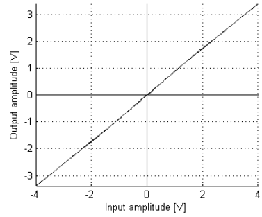
Fig. 10. Transfer function of amplifier I .
