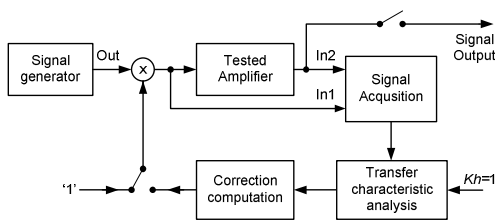
Fig. 4. Method of generating a corrected amplified signal.
