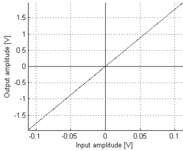
Fig. 14. Transfer function of amplifier II .
