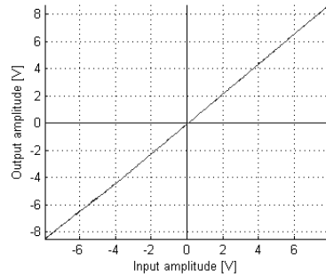
Fig. 18. Transfer function of amplifier III .
