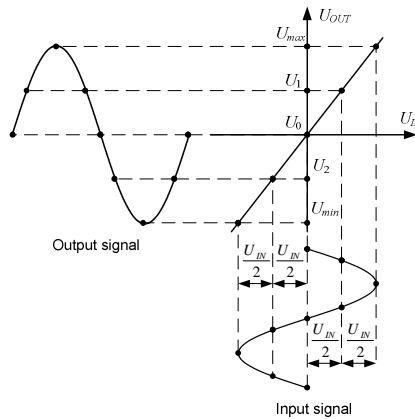
Fig. 2. Five ordinates method for THD marking.
