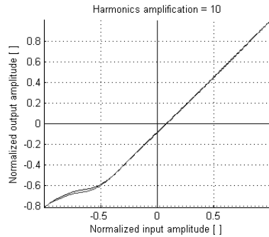
Fig. 19. Transfer function of amplifier III with amplified harmonics.
