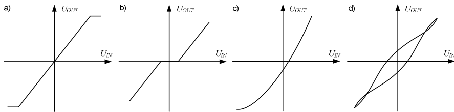
Fig. 1. Types of transfer function of signal amplifiers.
