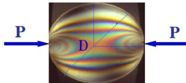
Fig. 2. Sample under compression.
