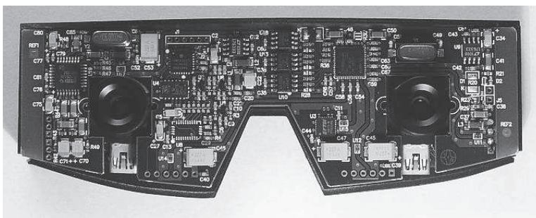
Fig. 1. A view of the hardware interface for the electronic travel aid for the blind.
