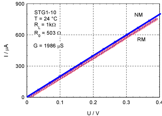
Fig. 4. The I - V characteristics for sample STG1-10 for NM and RM, measured at T = 24^\circ\text{C} .
