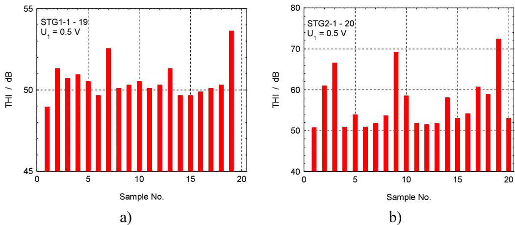
Fig. 11. The third index THI for samples of technology G – set STG1 (a) and set STG2 (b).
